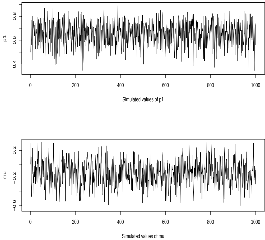
FIGURE 25.5. Simulated values of p_1 and \mu .
