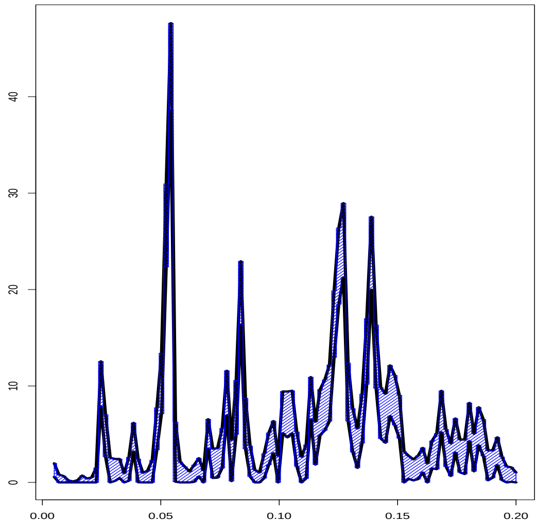
FIGURE 21.7. 95 per cent Confidence bands for kernel density estimate for the astronomy data.
