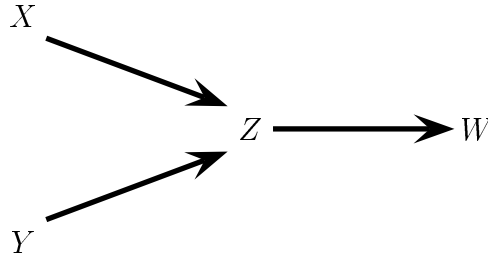
FIGURE 20.2. Another DAG.
