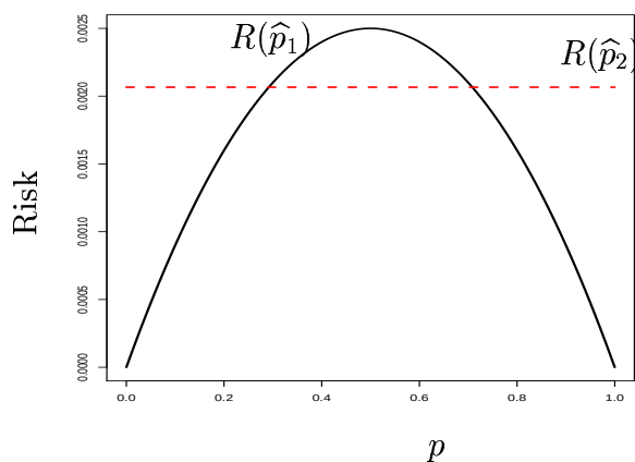
FIGURE 13.2. Risk functions for \hat{p}_1 and \hat{p}_2 in Example 13.3.
